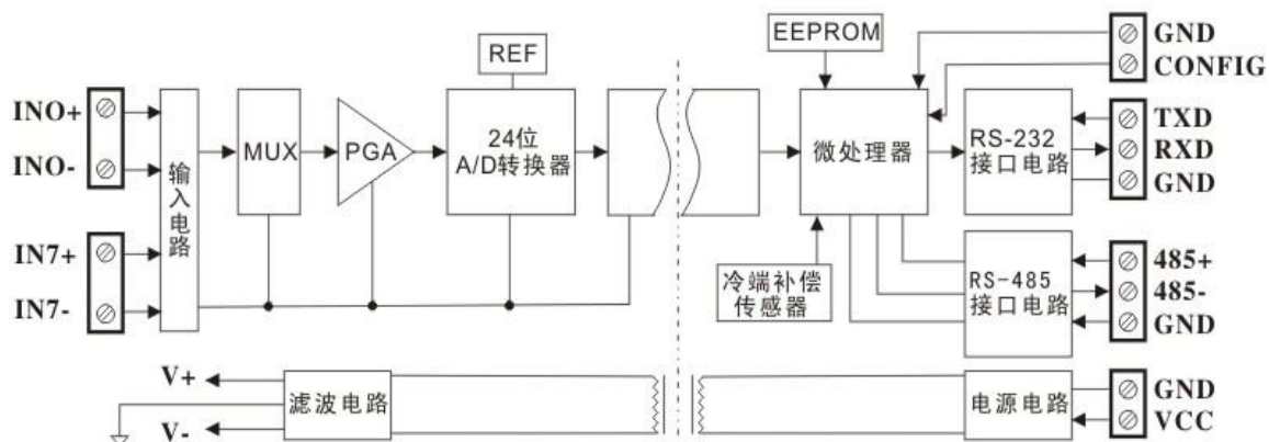
Fig.1 SYAD08T Thematic and External Terminal Diagram
